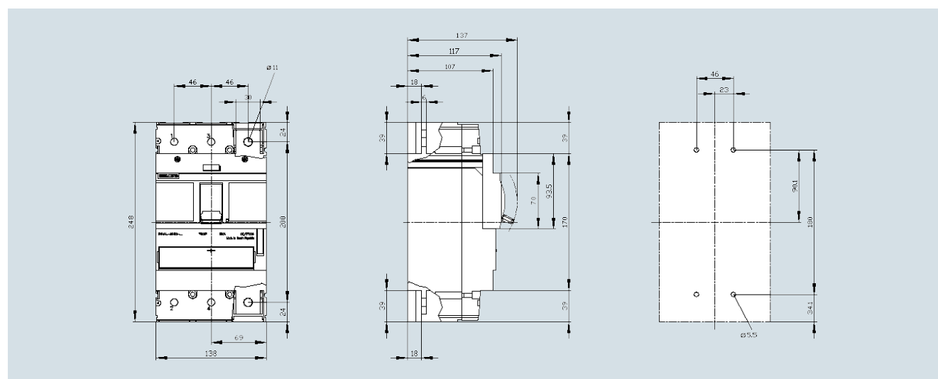
3VA13/14, 3-pole
